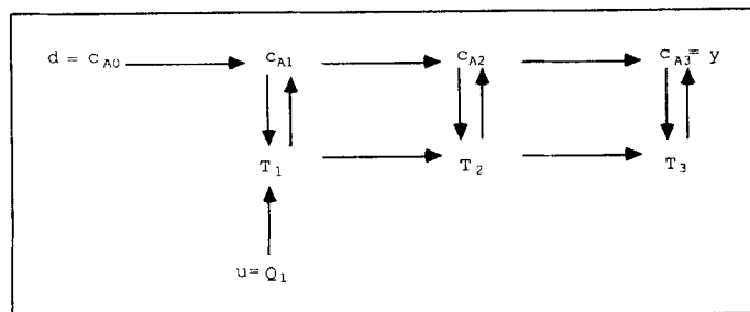
Figure 6. Interaction paths among process variables: Case 3.
