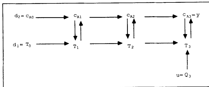
Figure 4. Interaction paths among process variables: Case 1.
